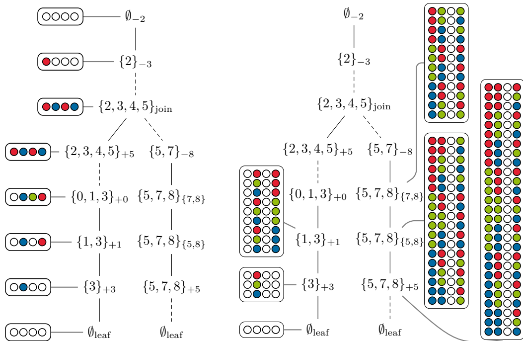
■ Figure 1 The left picture shows a part of a tree decomposition of the grid graph \begin{matrix} \circ & \circ & \circ \\ \circ & \circ & \circ \\ \circ & \circ & \circ \end{matrix} with vertices \{0, \dots, 9\} . The index of a bag shows the type of the bag: a positive sign means “introduce”, a negative one “forget”, a pair represents an “edge”-bag, and text is self explanatory. Solid lines represent real edges of the decomposition, while dashed lines illustrate a path (i. e., there are some bags skipped). On the left branch of the decomposition a run of a nondeterministic tree automaton with tree-index \begin{pmatrix} 0 & 1 & 2 & 3 & 4 & 5 & 6 & 7 & 8 \\ 2 & 3 & 0 & 1 & 2 & 3 & 0 & 1 & 0 \end{pmatrix} for 3-COLORING is illustrated. To increase readability, states of the automaton are connected to the corresponding bags with gray lines, and for some nodes the states are omitted. In the right picture the same automaton is simulated deterministically.
